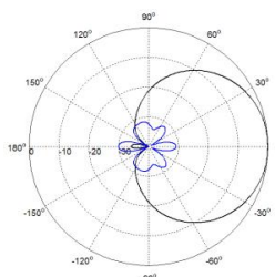
Azimuth(1710-2690MHz)
