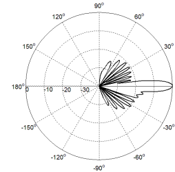
Elevation(1710-2690MHz)
